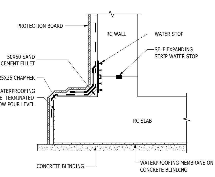
JOINT AT SLAB ON GRADE SCALE: N.T.S.
