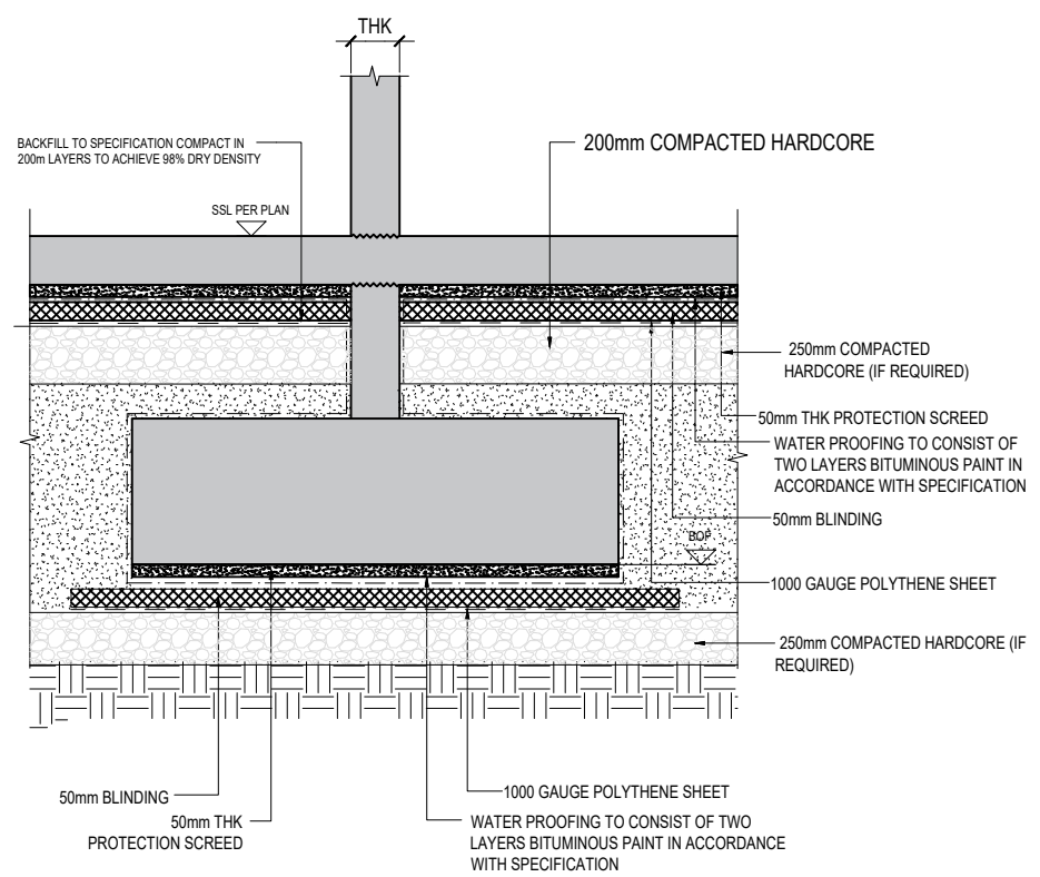
TYP. SLAB ON GRADE AND FOOTING WATERPROOFING LAYERS SCALE: N.T.S.
